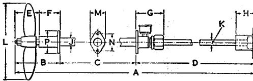
Dimensions of Standard Stern Gear
